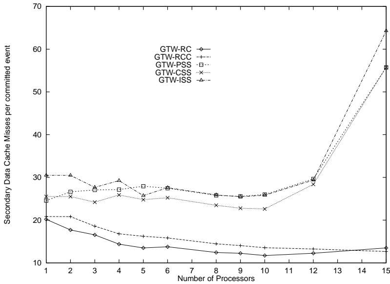
Fig. 11. Secondary data cache miss rate: reverse computation vs. state-saving on the PCS network model with 14,400 LPs.
