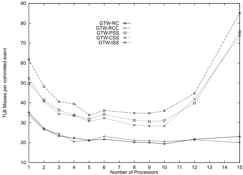
Fig. 12. TLB miss rate: reverse computation vs. state-saving on the PCS network model with 14,400 LPs.
