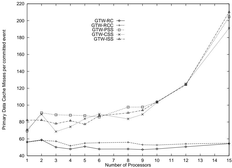
Fig. 10. Primary data cache miss rate: reverse computation vs. state-saving on the PCS network model with 14,400 LPs.
