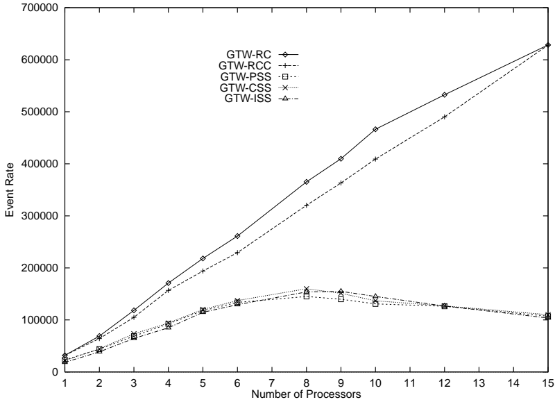
Fig. 9. Event rate: reverse computation vs. state-saving on the PCS network model with 14,400 LPs.
